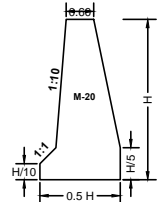
TYPICAL C/S OF SQUARE RETURN
