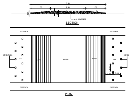
DETAILS OF RAISED PEDESTRAIN CROSSING
