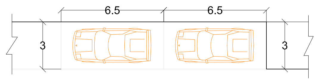
PARKING DIMENSIONS FOR 4 WHEELERS
