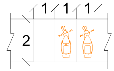
PARKING DIMENSIONS FOR 2 WHEELERS
