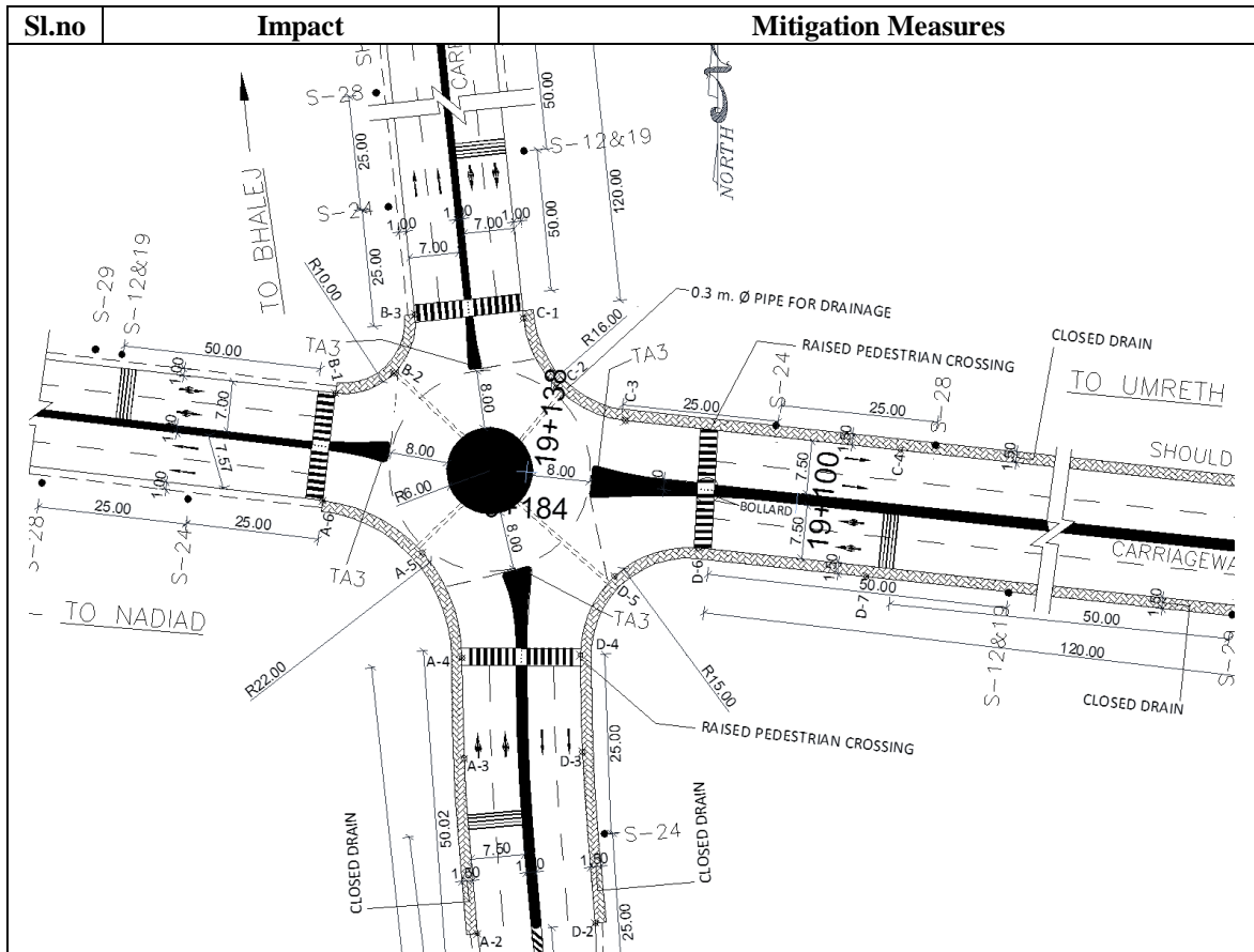
Junction Design at Sarsa (Ch 19+130)
