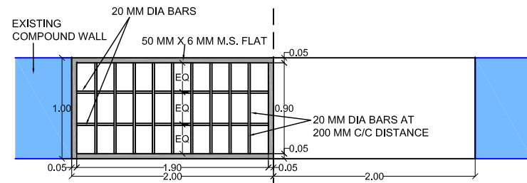
PROPOSED GATE AS PER DESIGN SCALE: NTS
