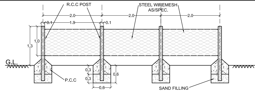
CHAIN FENCING AS PER DESIGN SCALE: NTS
