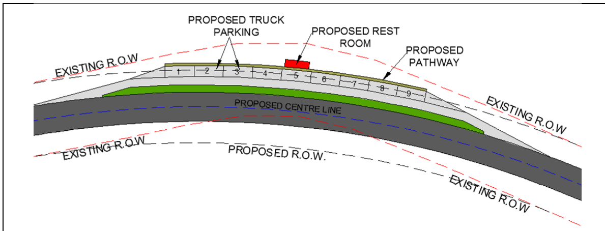
Figure 2.2: Conceptual Sketch of Truck Layby parking area from chainage 230+275 to 230+500
