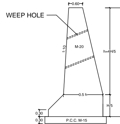
TYPICAL SECTION OF R.WALL
