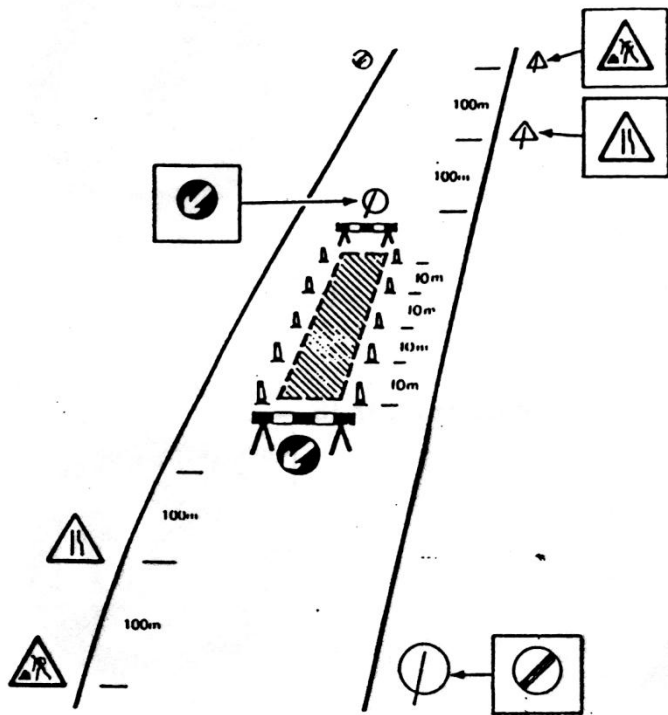
Sign layout for centre line working (drawn for driving on the left)
